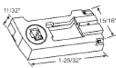
83-500 White Cam. Opening: 1/4" x 3/16" Used with Pivot Bar 83-504
