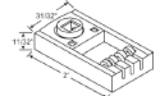
83-510 Opening: 9/32" x 7/32"
