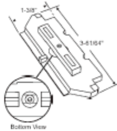
900-8600MOD Black with springs. Modified to accept tamper proof screw. Traco
