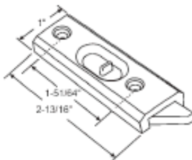
85-511 Tilt Tensioning Tool Used with 83 and 85 Series Balances
