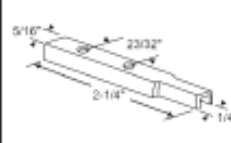
85-557 Stamped. Use with 83-505 Pivot Lock Shoe. Rollyson
