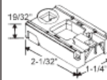
85-517 Black Cam Cam Opening: 3/8" x 3/16"
