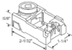
85-525 Green Cam Cam Opening: 5/16" x 3/16" Thermalgard
