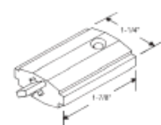
85-525 Green Cam Cam Opening: 5/16" x 3/16" Thermalgard
