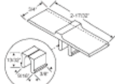
900-8600 Black with springs. Used with pivot bar 900-8599. Traco
