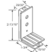
900-18899 White, Plastic Acro/Slocomb
