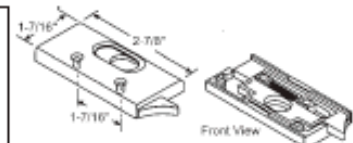
900-21112 Black Anodized Aluminum
